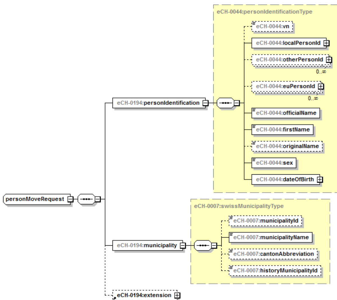
Figure 6: personMoveRequest
