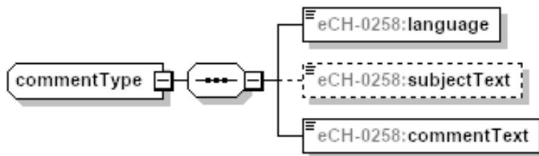
Figure 15: commentType
