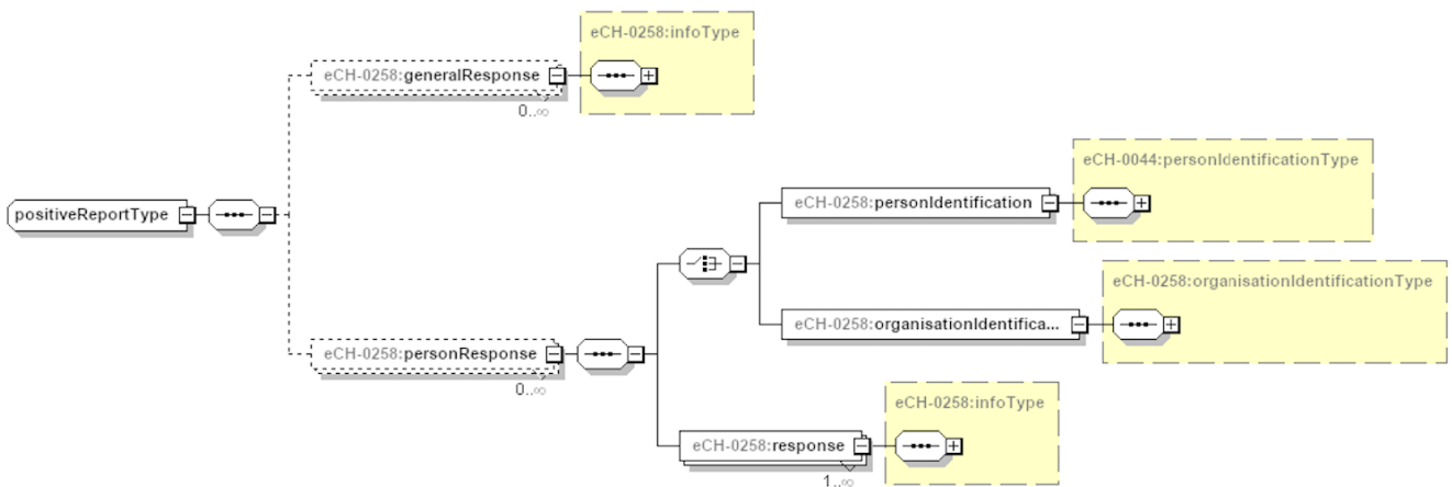
Figure 17: positiveReportType
