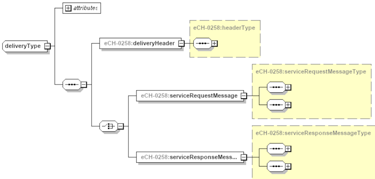
Figure 25: deliveryType
