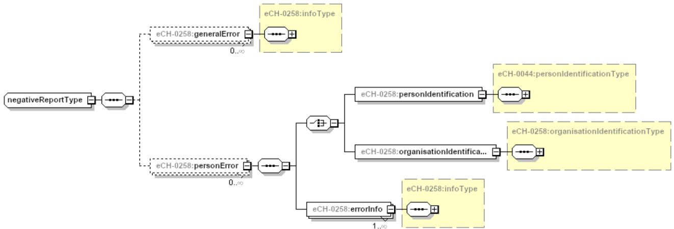
Figure 18: negativeReportType
