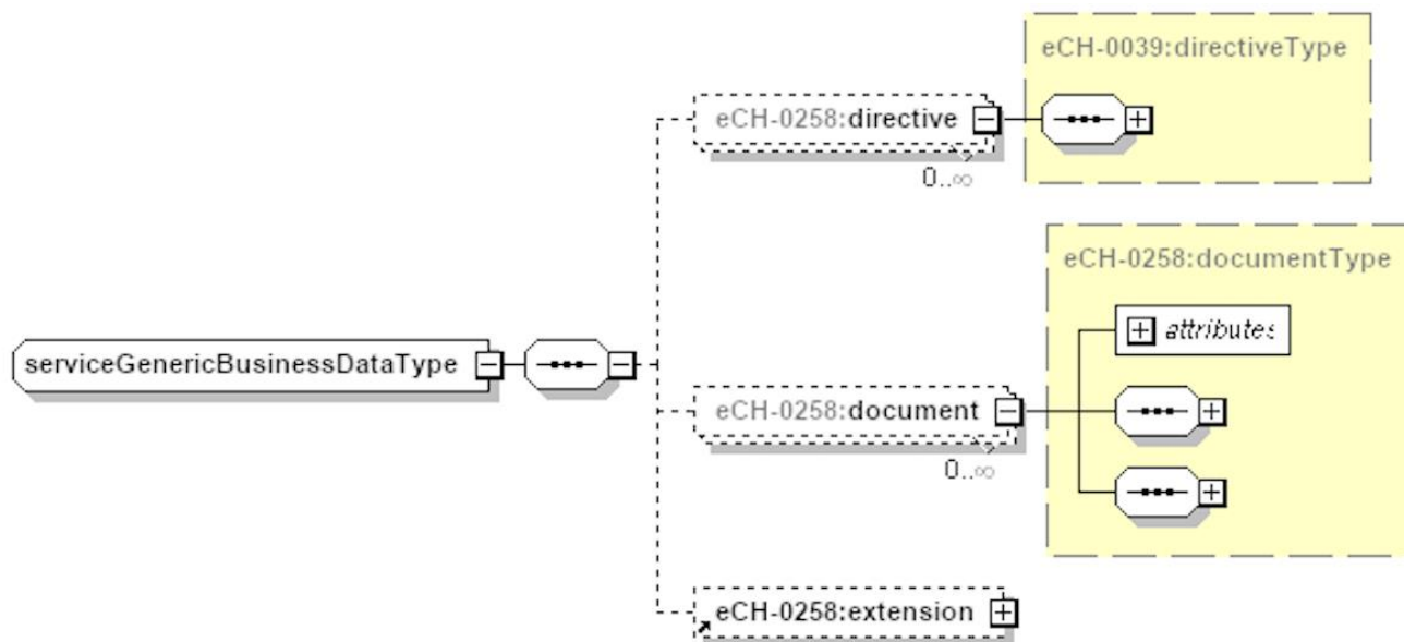
Figure 12: serviceGenericBusinessDataType
