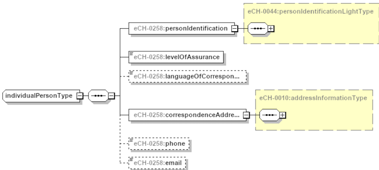
Figure 8: individualPersonType
