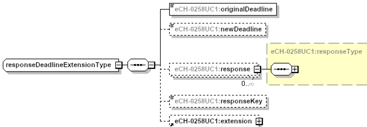
Figure 21: deadlineExtensionResponseType
