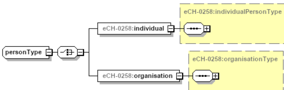
Figure 7: personType
