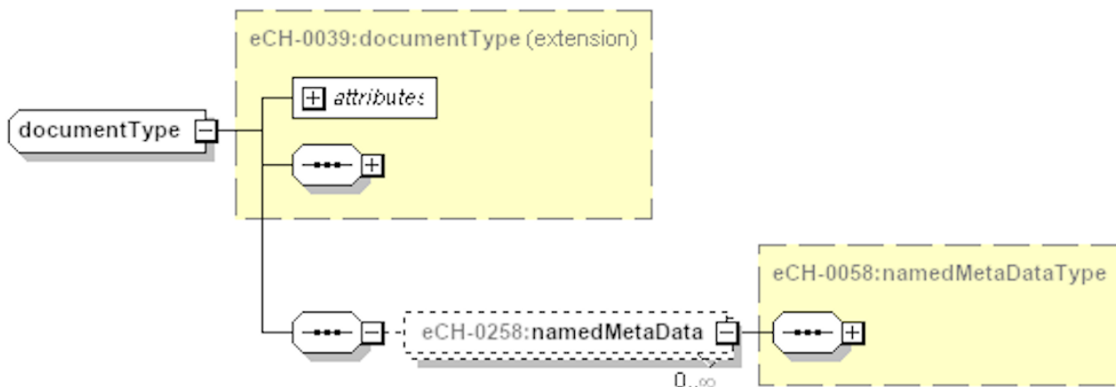
Figure 13: documentType
