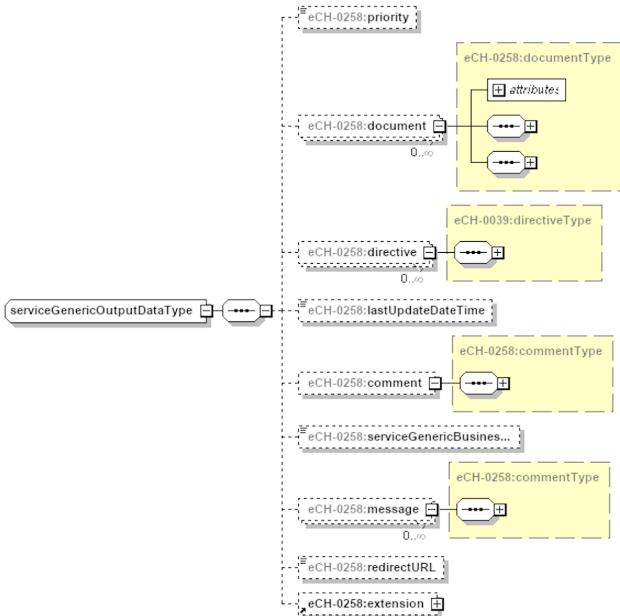
Figure 14: serviceGenericOutputDataType
