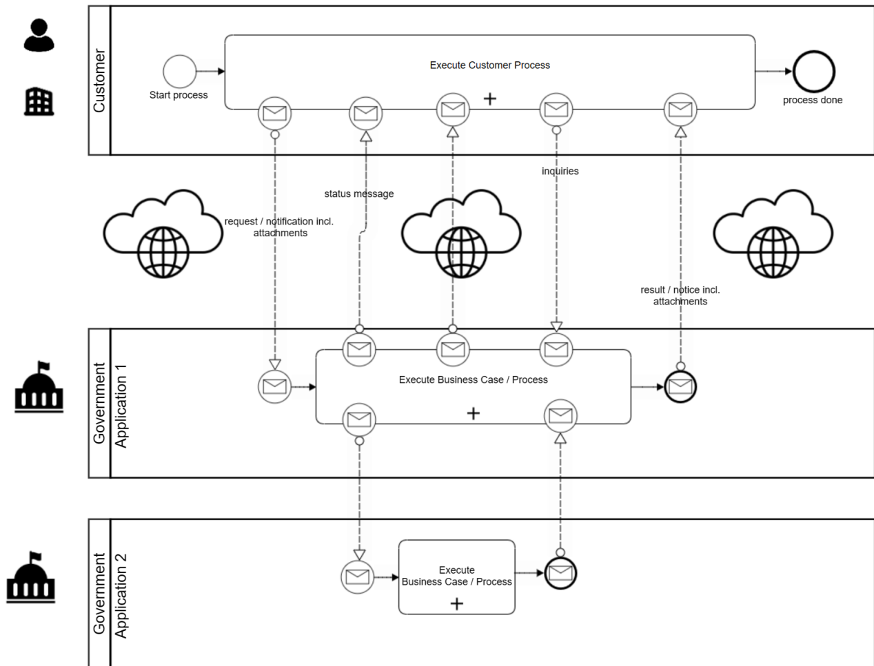
Figure 1: Champ d'application
