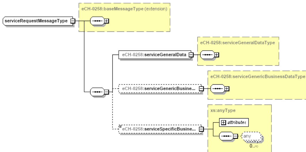
Figure 23: serviceRequestMessageType
