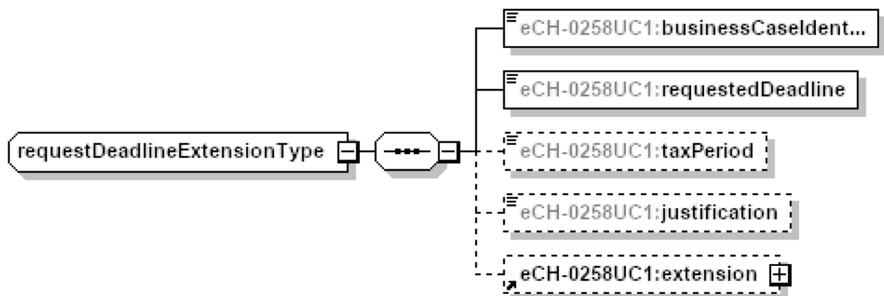
Figure 20: requestDeadlineExtensionType
