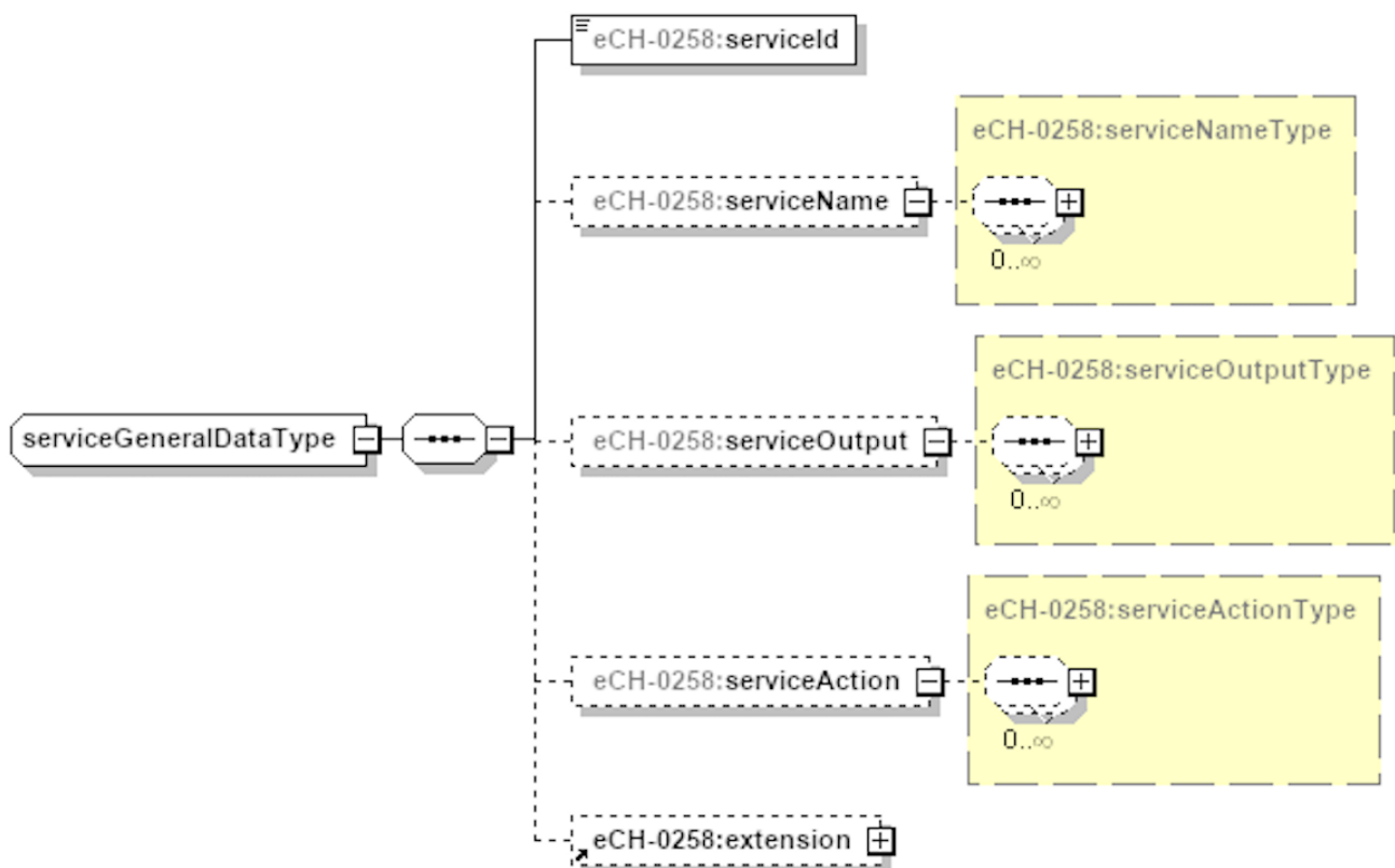
Figure 11: serviceGeneralDataType
