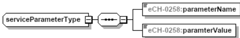
Figure 16: serviceParameterType
