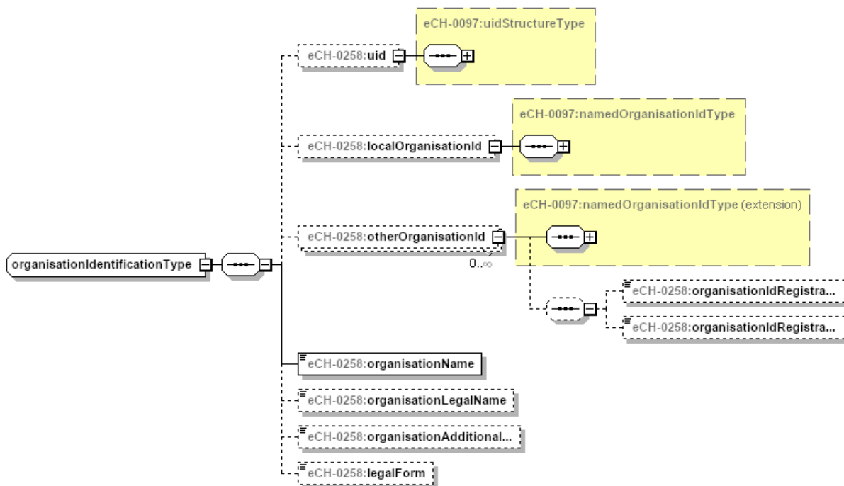
Figure 10: organisationIdentificationType
