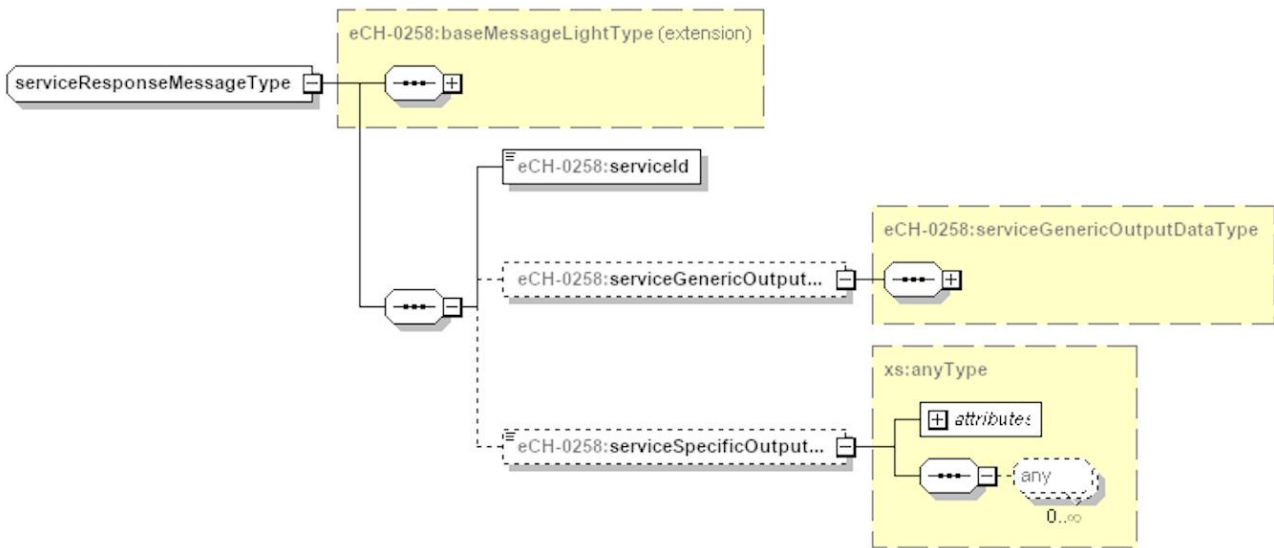
Figure 24: serviceResponseMessageType
