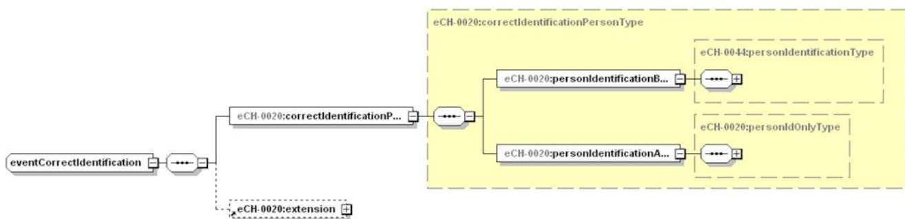
Figure 71: eventCorrectIdentification
