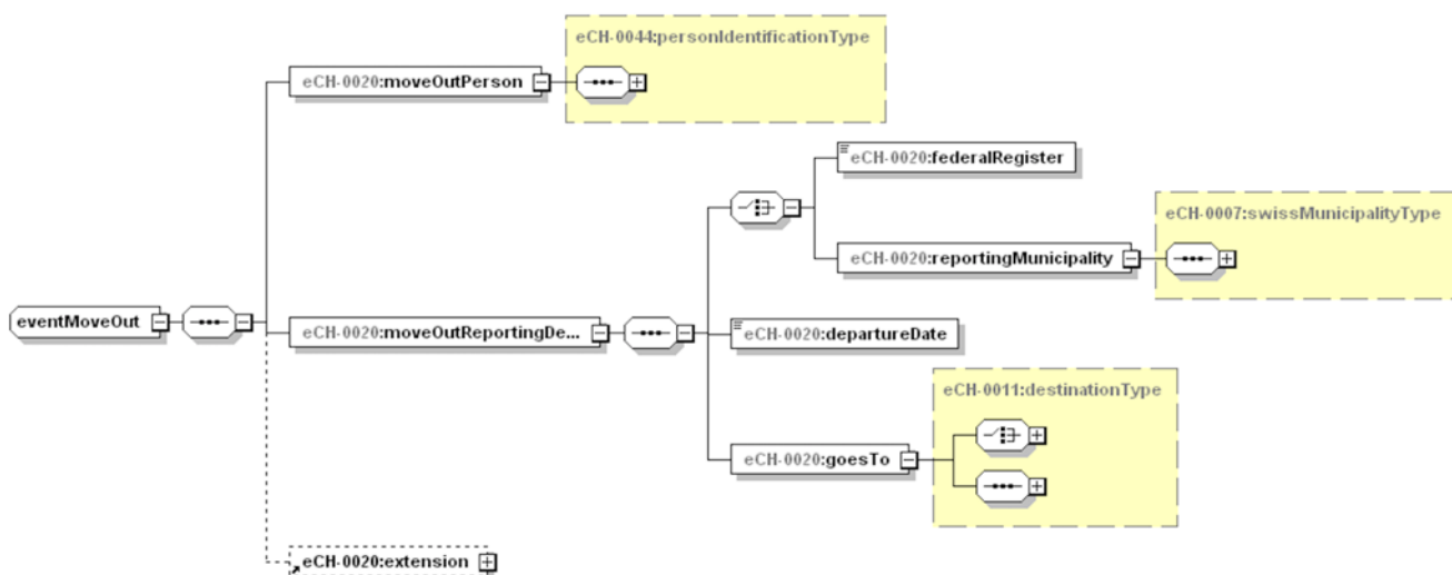
Figure 46: eventMoveOut
