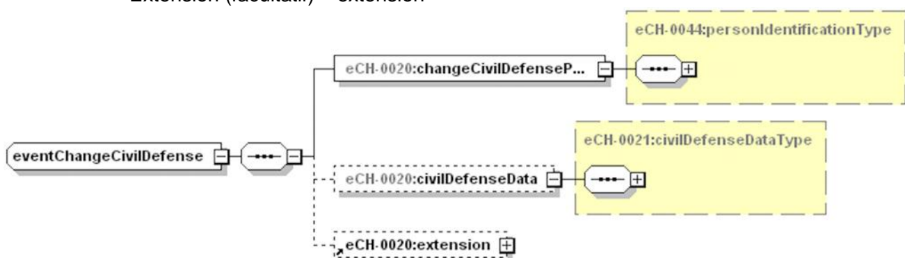
Figure 63: eventChangeCivilDefense
