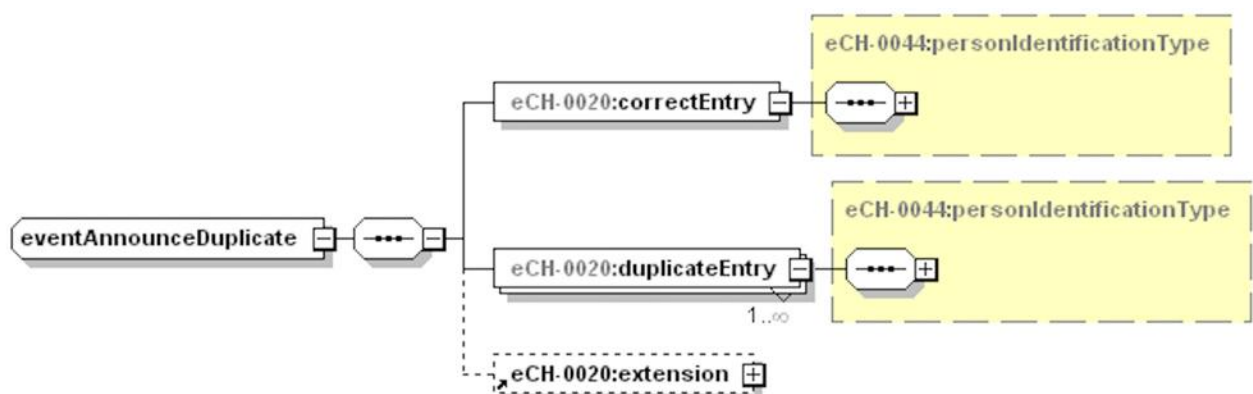
Figure 19: eventAnnounceDuplicate
