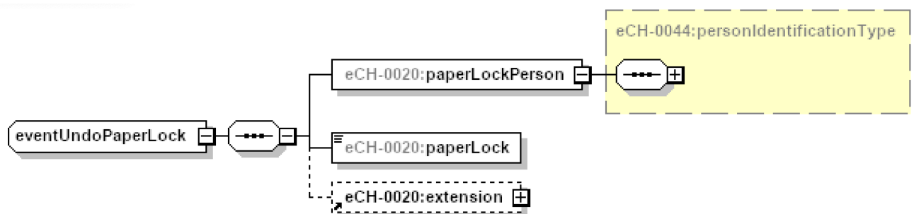
Figure 60: eventUndoPaperLock
