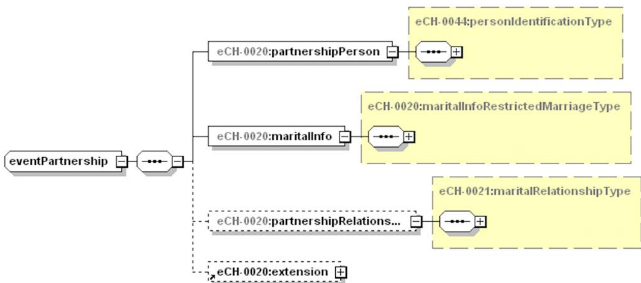
Figure 30: eventPartnership
