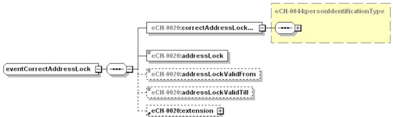
Figure 82: eventCorrectAddressLock
