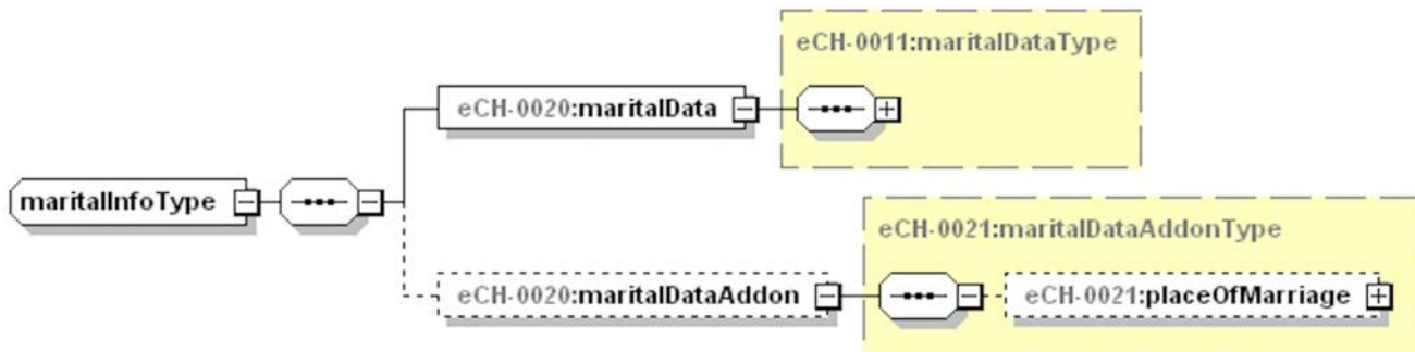
Figure 5: maritalInfoType
