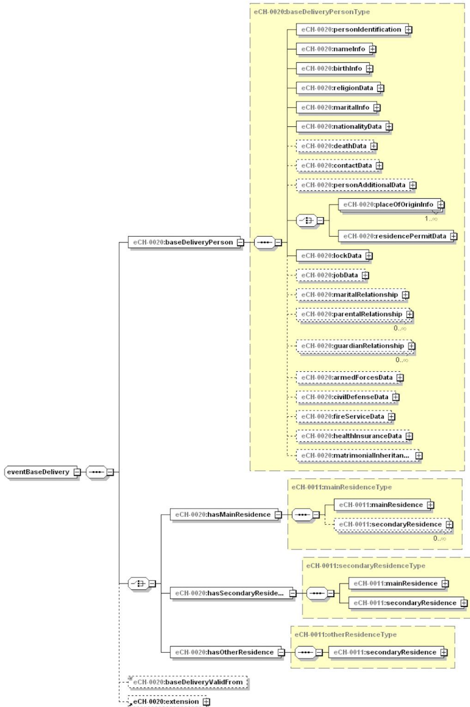
Figure 15: eventBaseDelivery
