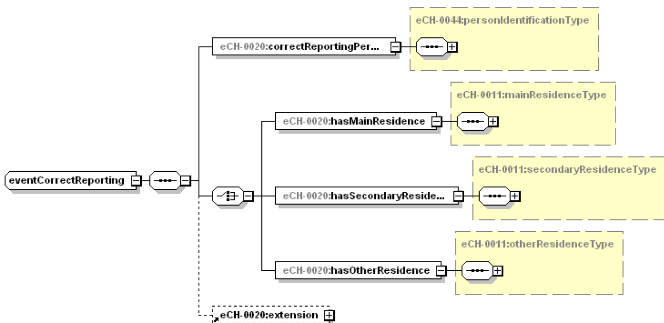
Figure 69: eventCorrectReporting
