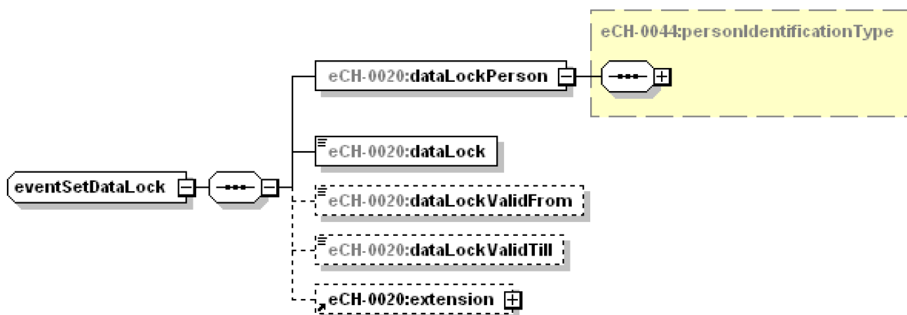
Figure 57: eventSetDataLock
