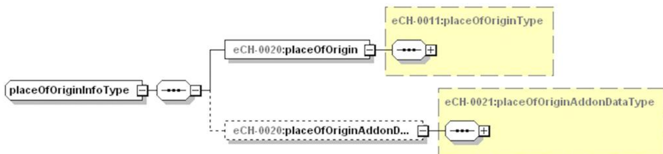
Figure 7: placeOfOriginInfoType
