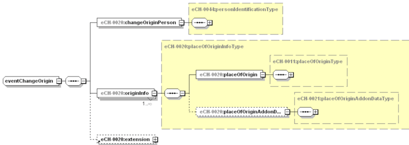
Figure 27: eventChangeOrigin
