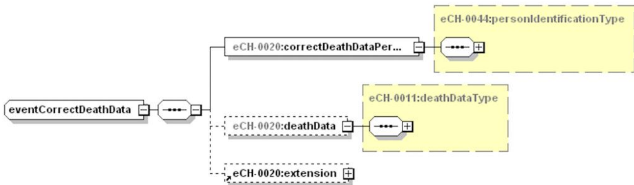
Figure 80: eventCorrectDeathInfo
