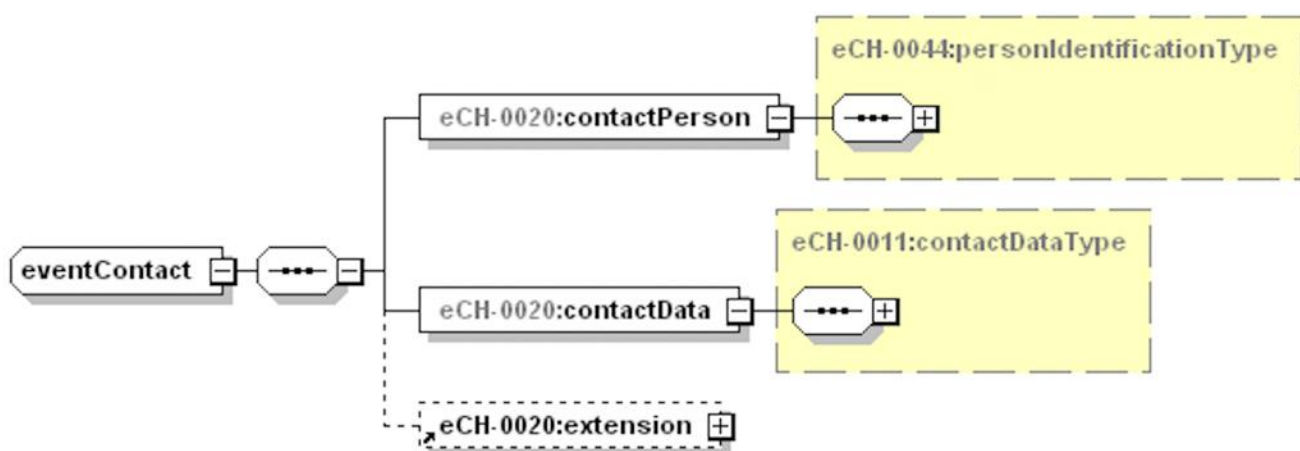
Figure 44: eventContact
