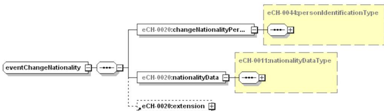
Figure 53: eventChangeNationality
