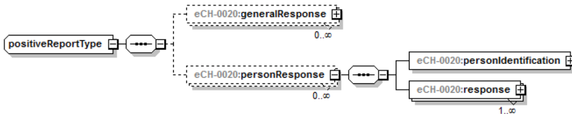
Figure 12: positiveReportType
