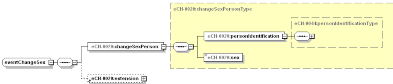
Figure 41: eventChangeSex
