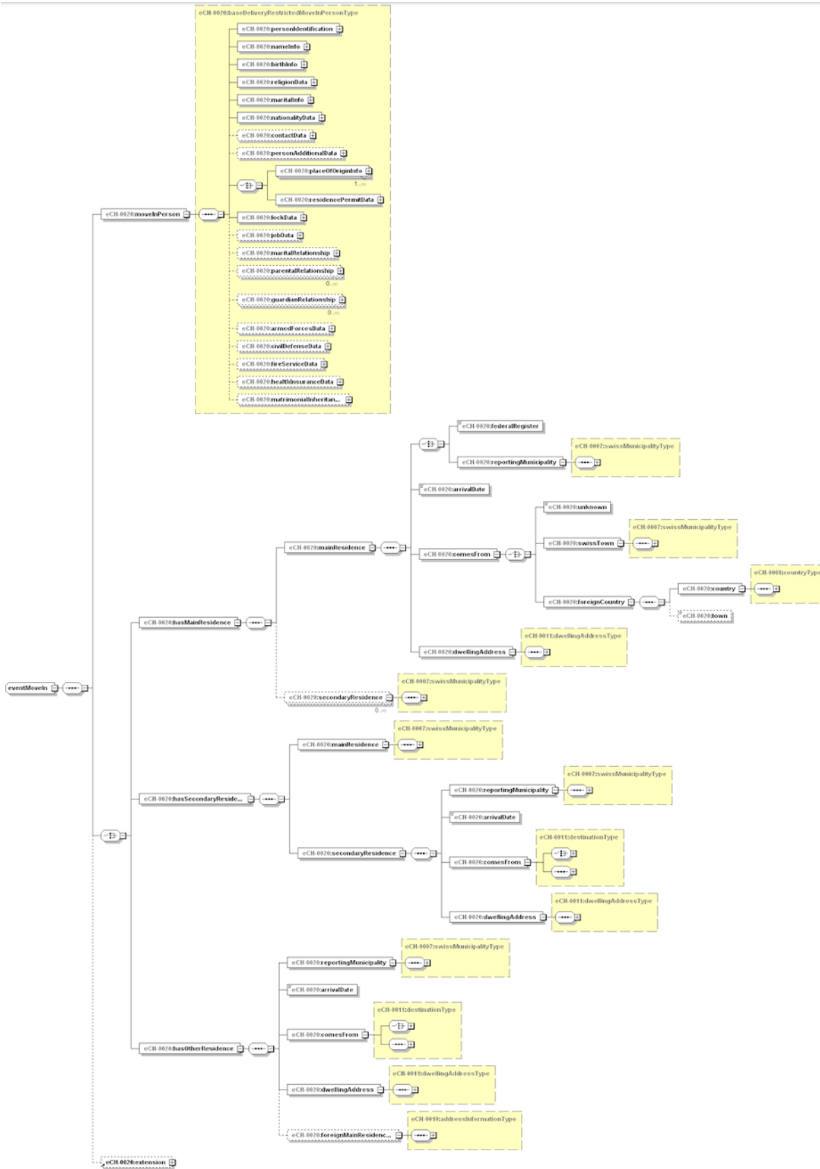
Figure 42: eventMoveIn
