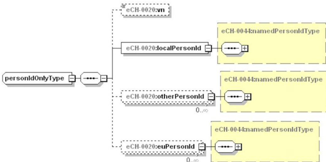
Figure 2: personOnlyType
