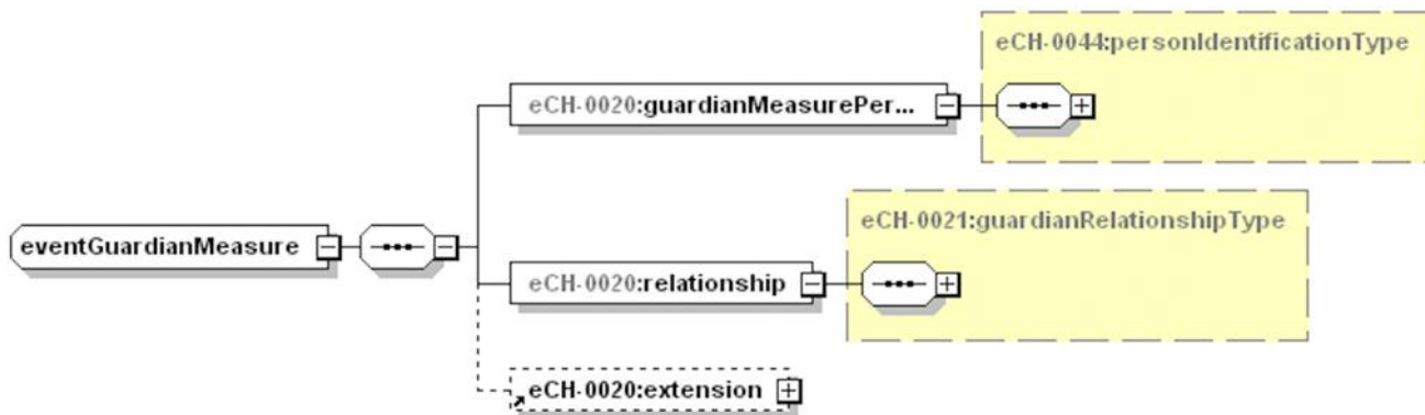
Figure 50: eventGuardianMeasure
