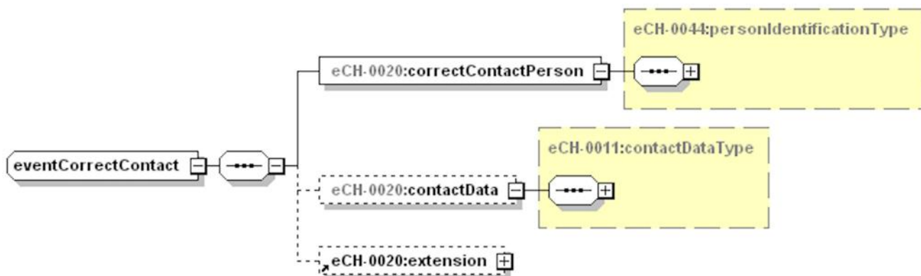
Figure 74: eventCorrectContact
