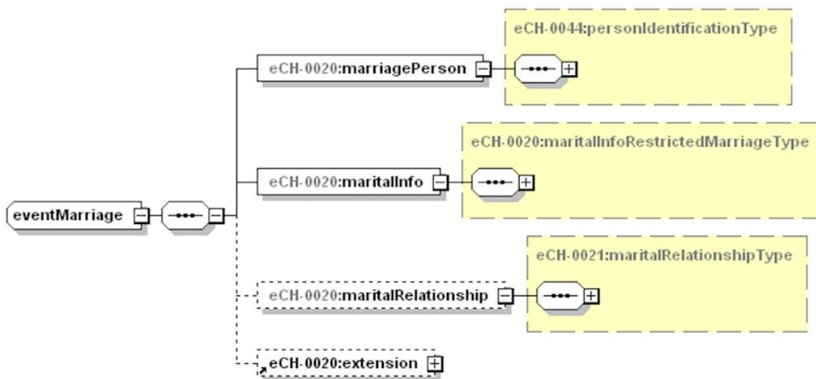
Figure 29: eventMarriage
