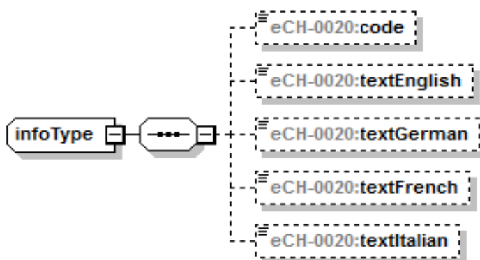
Figure 14: infoType
