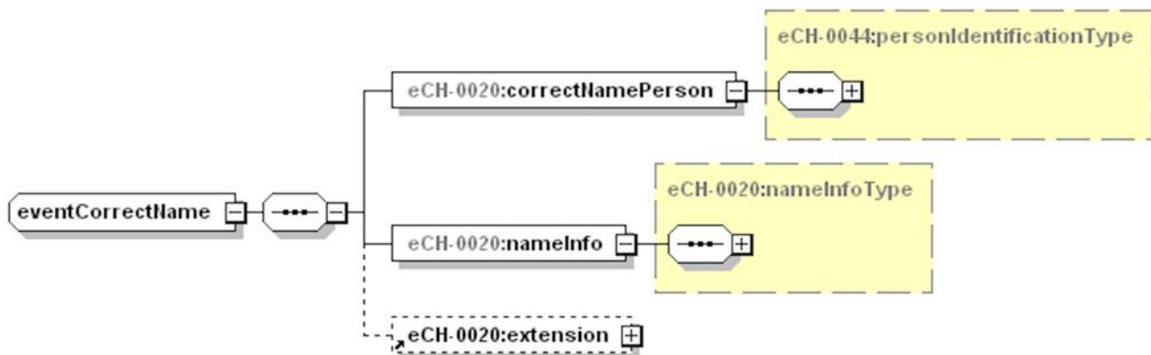
Figure 72: eventCorrectName
