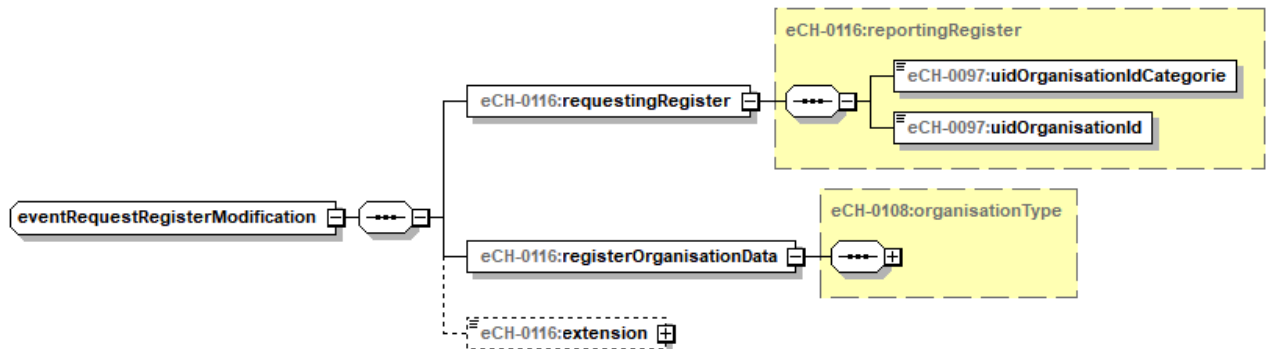
Figure 10: eventInfoRegisterModification
